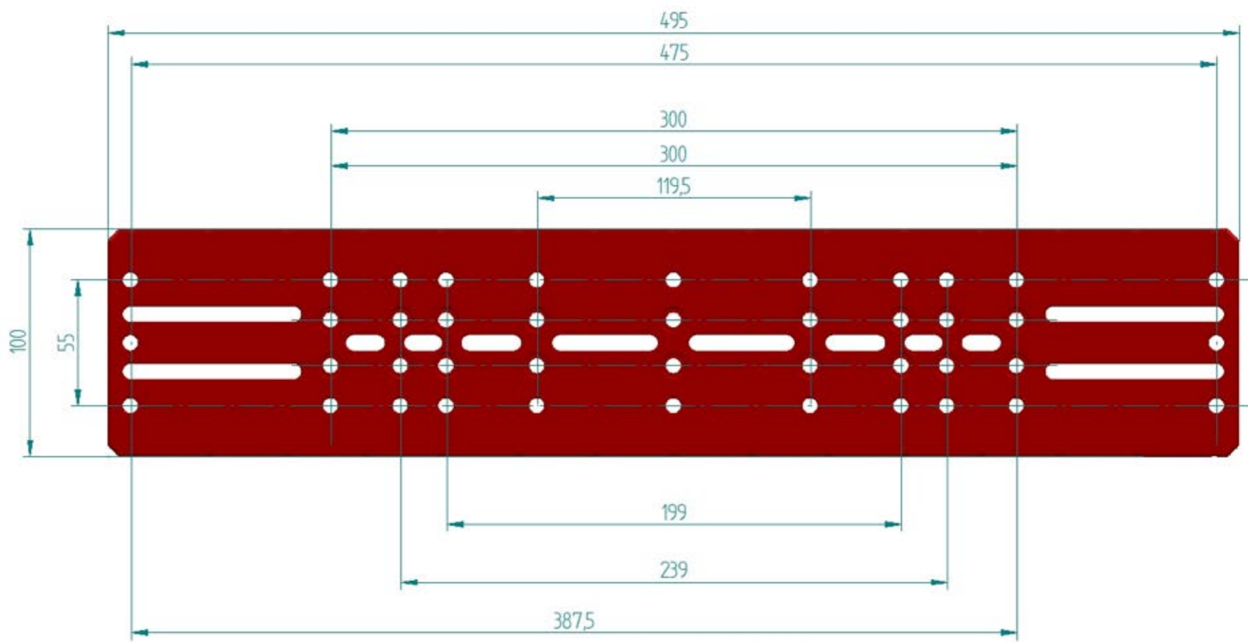
TOP VIEW
